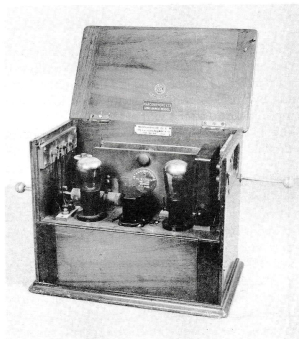
14 Wireless receiver model V2A of 1922
