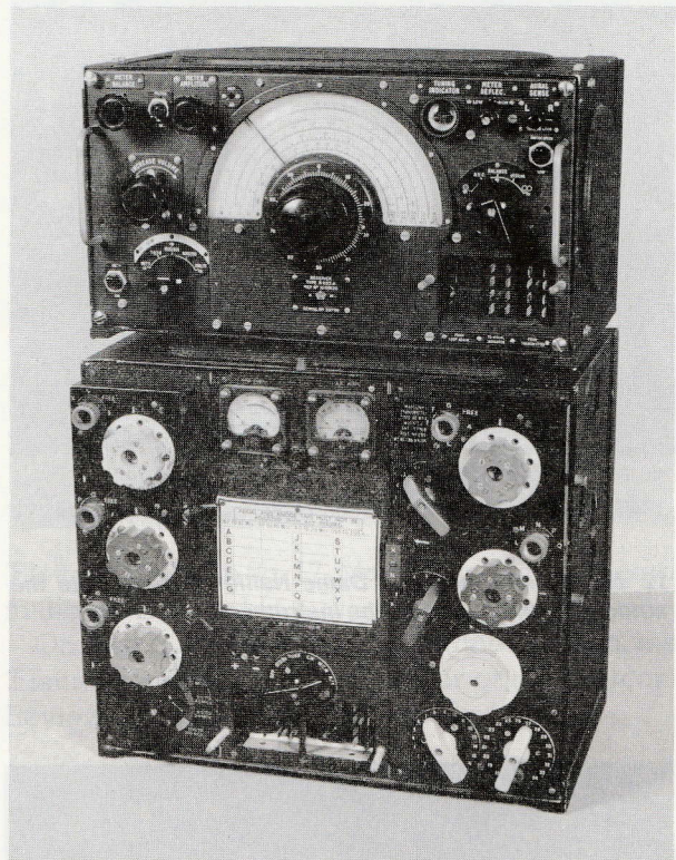
11 Transmitter and receiver units, T1154/R1155, of 1940
