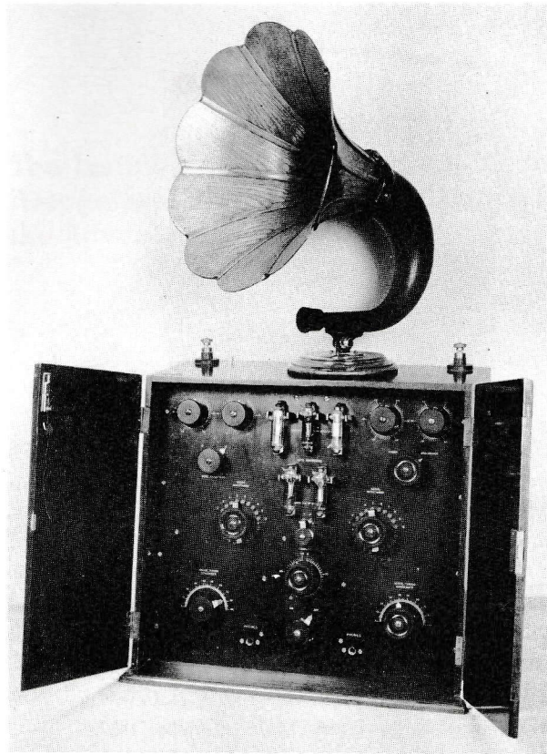
15 Wireless receiver and loudspeaker c.1925
